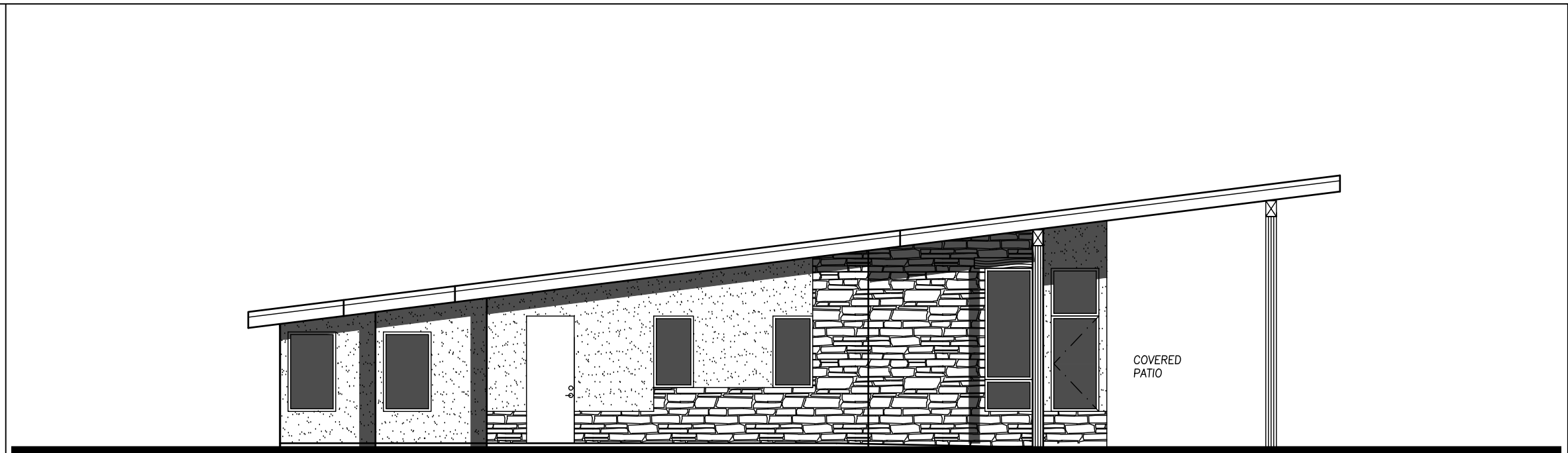
SOUTH ELEVATION
