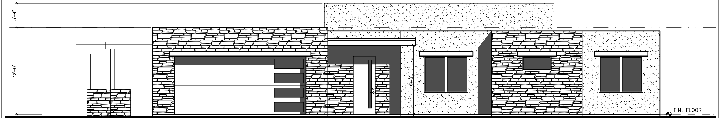
SOUTH ELEVATION
