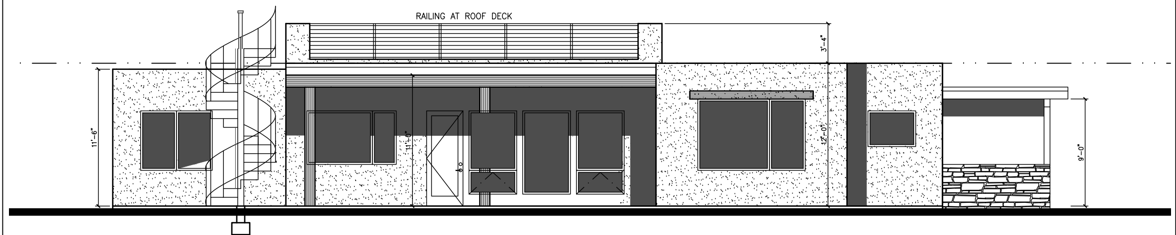
NORTH ELEVATION
