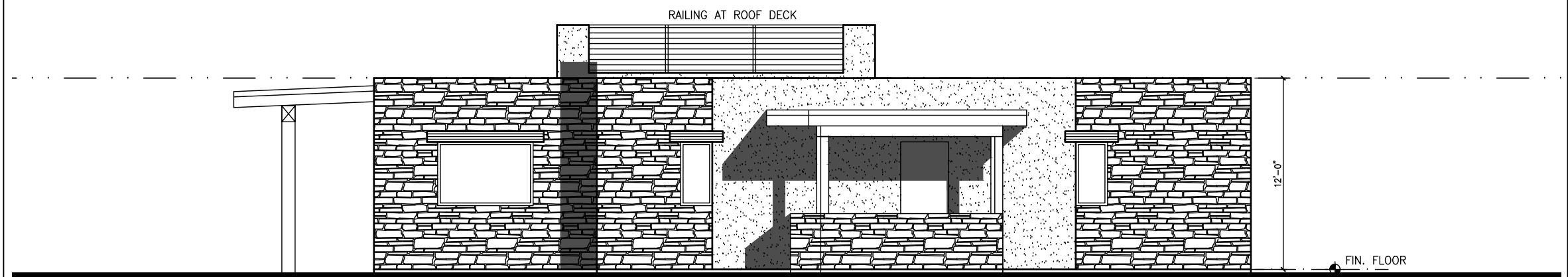
WEST ELEVATION
