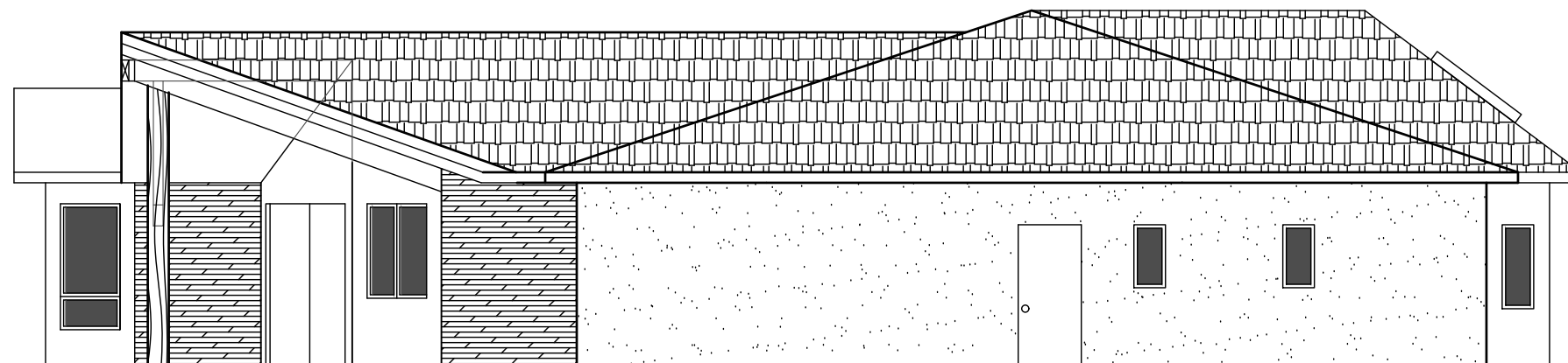
REAR ELEVATION
